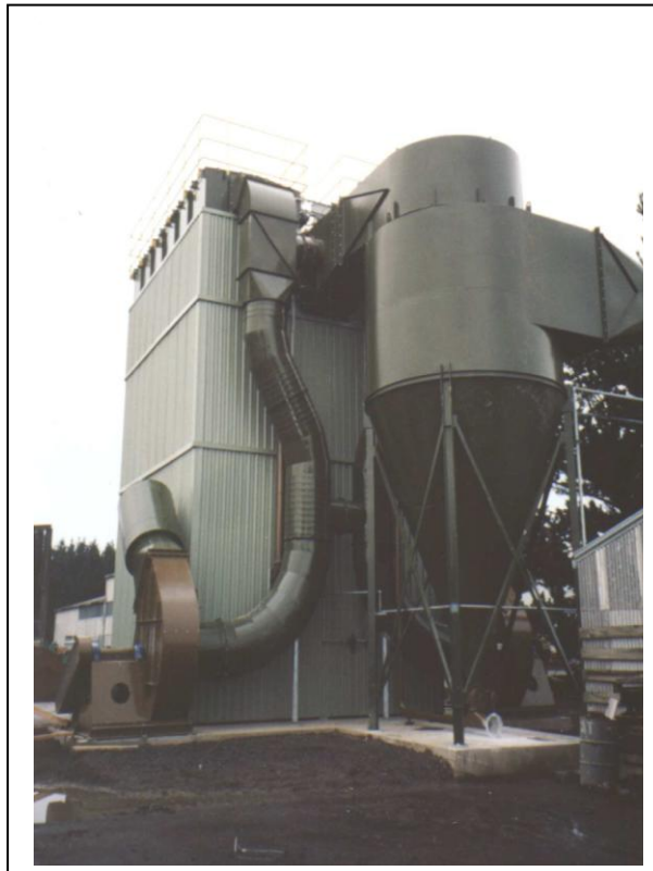
McKechnie metals high temperature smelter fume Pulse Jet Filter complete with grit arrestor
