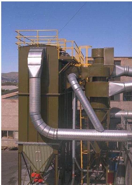
AW Frazer high temperature smelter baghouses complete with grit arrestor
